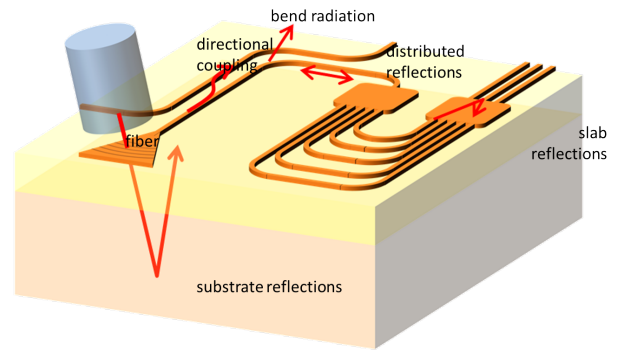
Fig. 2. High contrast photonic circuits will invariably suffer from parasitics: light which is reflected and scattered may interfere with the useful signals.
